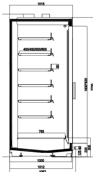
ROCK L ECO 20 FLAT CANOPY SQUARE S/S BUMPER
