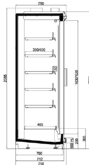
ROCK C ECO 20 CURVED CANOPY PVC BUMPER
