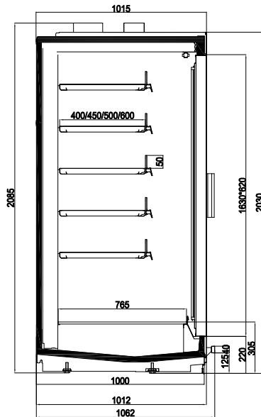
ROCK L ECO 20 FLAT CANOPY SQUARE S/S BUMPER
