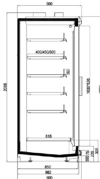
ROCK N ECO 20 CURVED CANOPY PVC BUMPER
