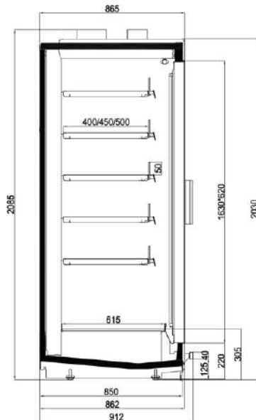
ROCK N ECO 20 FLAT CANOPY SQUARE S/S BUMPER
