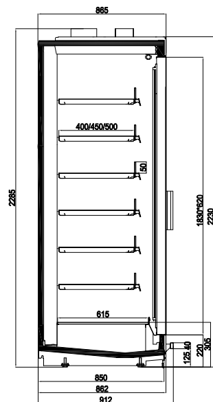
ROCK N ECO 20 FLAT CANOPY SQUARE S/S BUMPER
