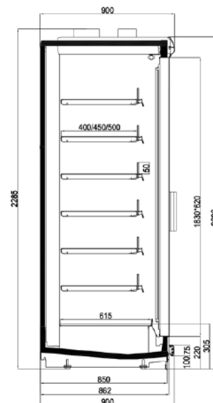
ROCK N ECO 20 CURVED CANOPY PVC BUMPER
