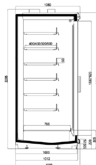
ROCK L ECO 22 CURVED CANOPY PVC BUMPER
